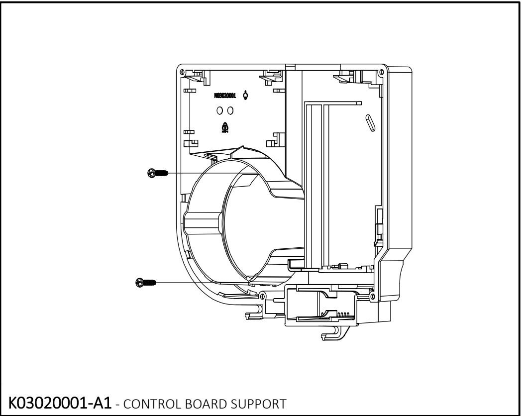
K03020001-A1 - CONTROL BOARD SUPPORT
