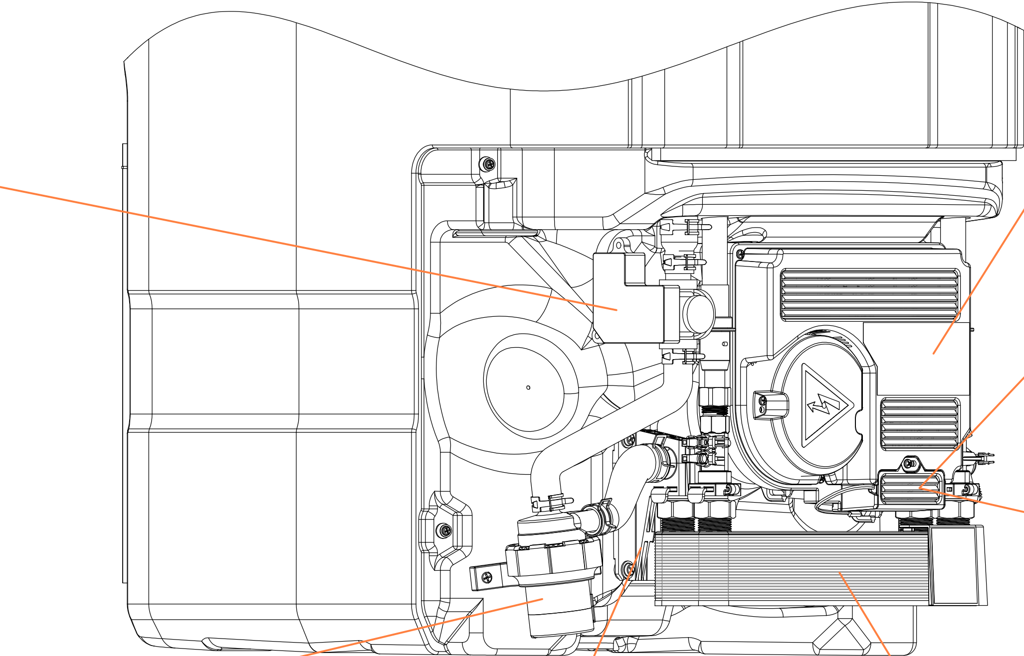
K01140000-A1 - OVERALL PRODUCT HOSES KIT (EXCEPT FILLING HOSE, SEE K01140003 KIT)
